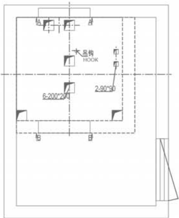
机房留孔图 CUTOUTS OF MACHINE ROOM
