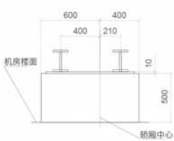
B-B承重墩 B-B BEARING HOLE
