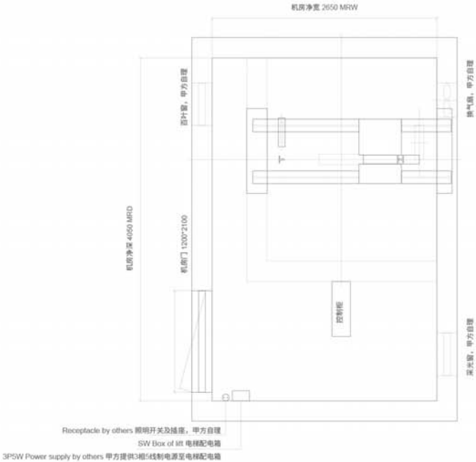
机房平面图 MACHINE ROOM PLAN
